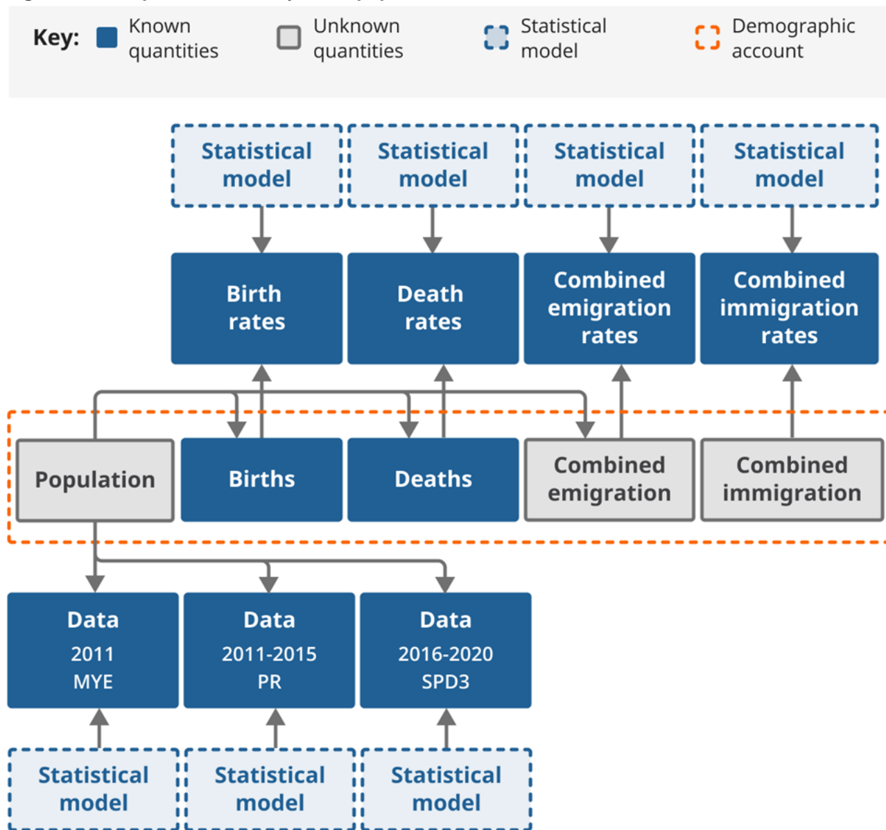
Figure 11: Components of the dynamic population model
