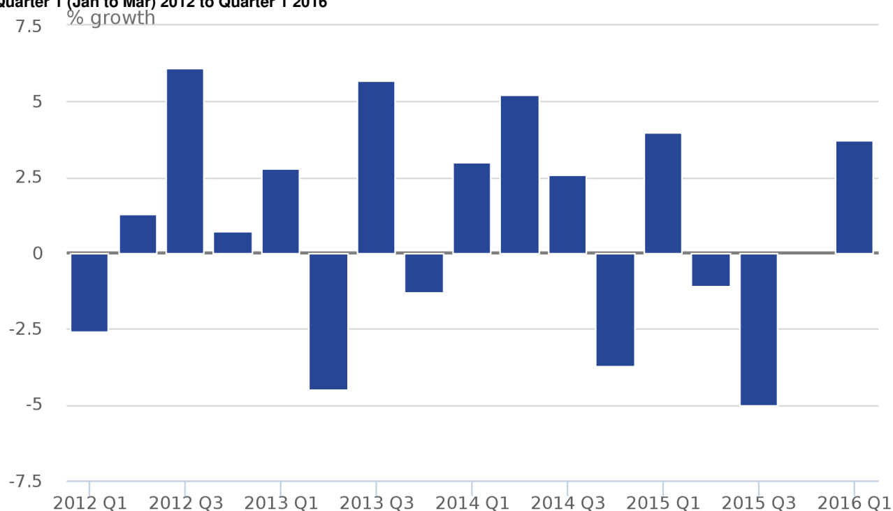
Figure 15: UK gross operating surplus of corporations' growth, quarter-on-quarter
